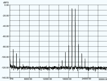
Graph 5. IMD (19/20kHz 1:1) at 1-watt into an 8-ohm non-inductive load
