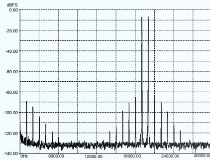
Graph 6. IMD (19/20kHz 1:1) at 20-watts into an 8-ohm non-inductive load
