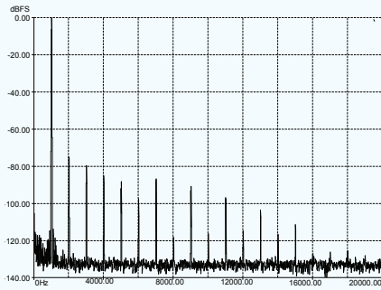
Graph 4. THD at 1kHz at 20-watts into a 4-ohm non-inductive load
